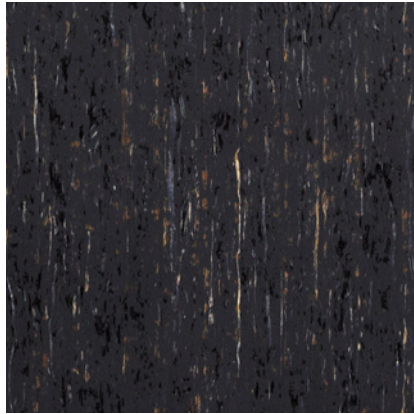
Cosmos
